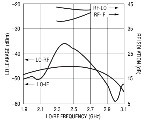
LO Leakage and RF Isolation vs LO and RF Frequency
